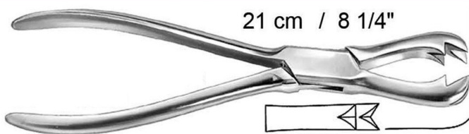
21 cm / 8 1/4" DMI-1981-482 Fergusson Bone Holding Forceps Heavy pattern
