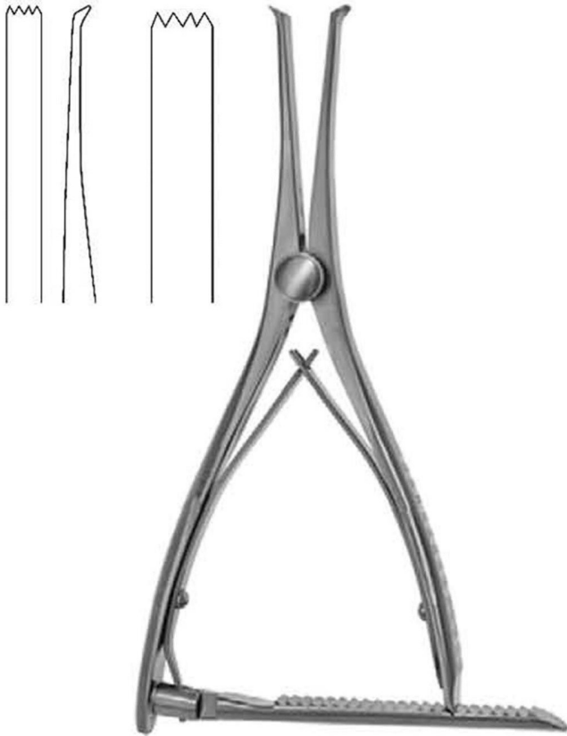
DMI-1981-584 Vertibra Spreader / Retractor A: 18 cm / 7" | B: 28 cm / 11"
