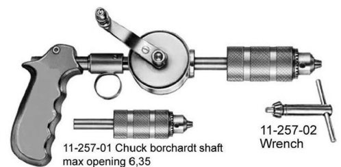
DMI-1981-056 Martin Hand Drill with Chuck & Wrench
